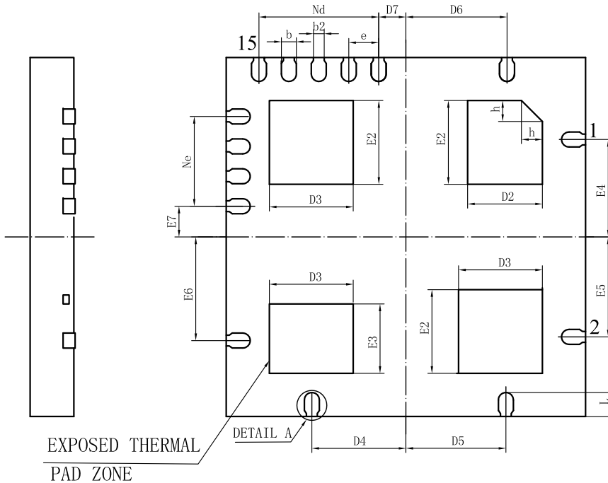
BOTTOM VIEW
