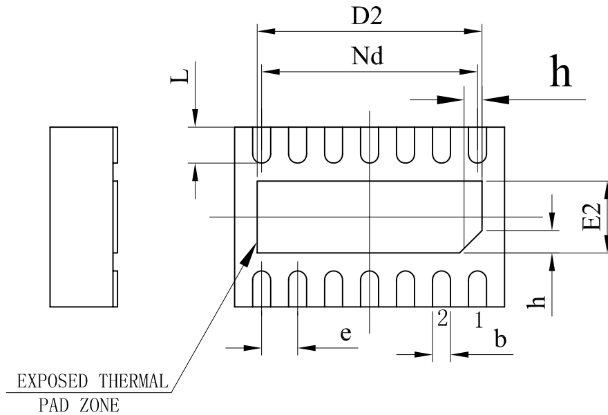
BOTTOM VIEW
