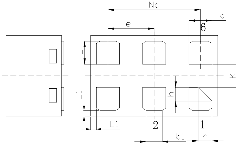
BOTTOM VIEW
