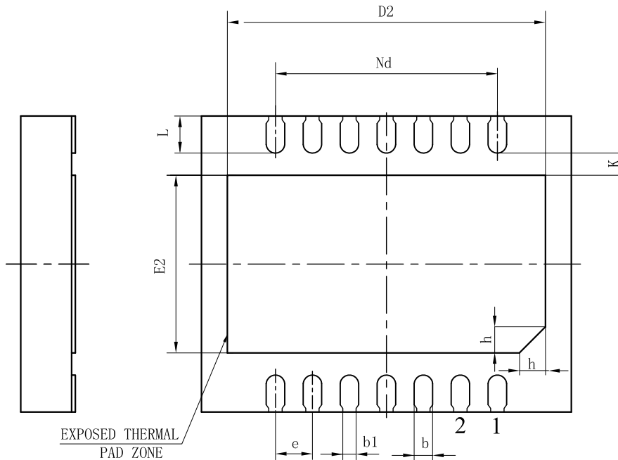
BOTTOM VIEW
