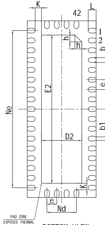
BOTTOM VIEW
