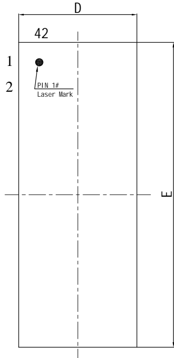
TOP VIEW
