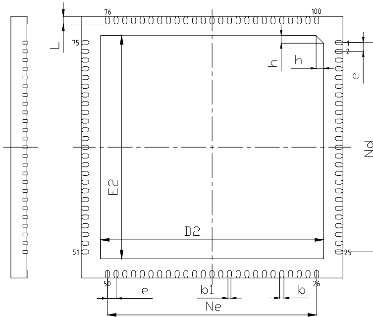
BOTTOM VIEW
