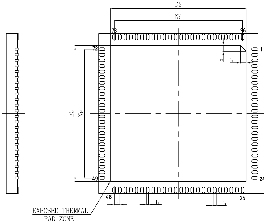
BOTTOM VIEW
