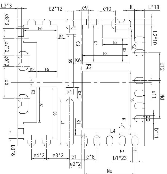
BOTTOM VIEW
