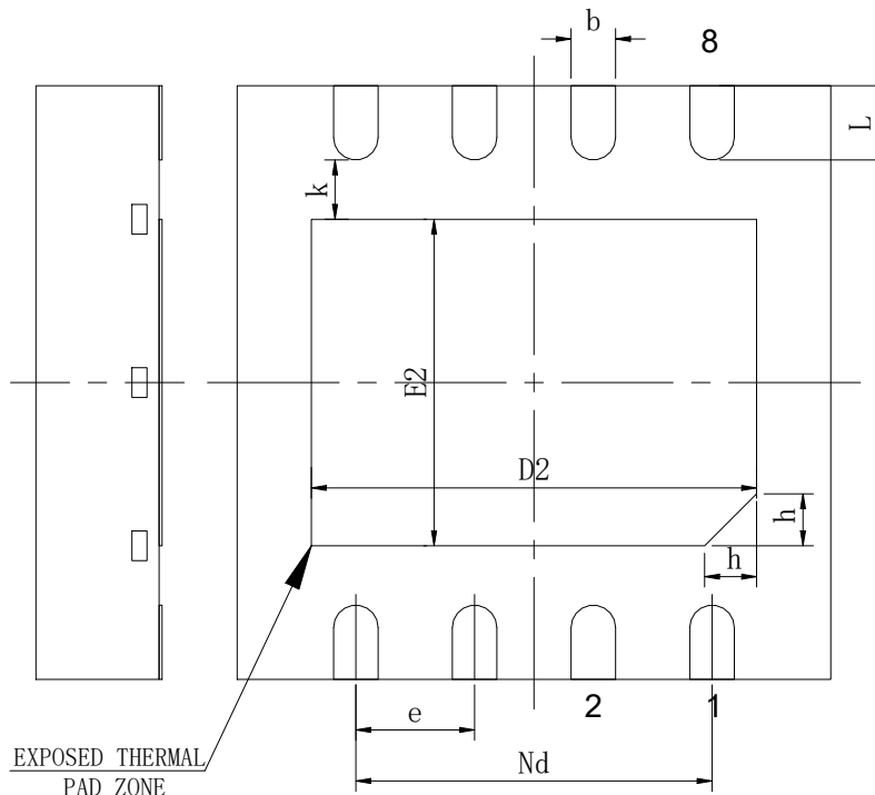
BOTTOM VIEW
