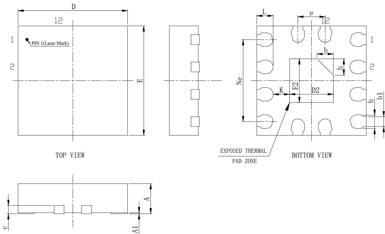
SIDE VIEW
