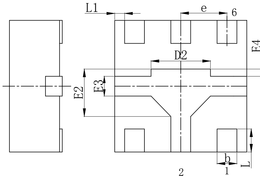
2 1 BOTTOM VIEW
